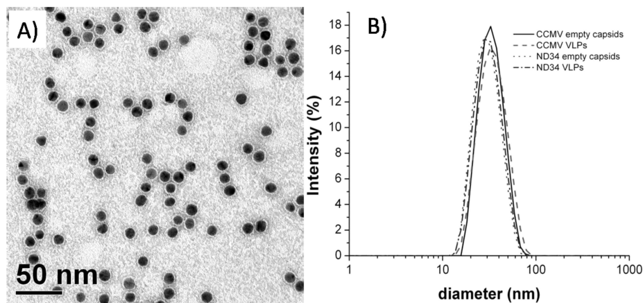
Figure 1. Formation of \Delta 34 and CCMV VLPs using TEG-coated gold nanoparticles cores. (A) TEM image of 11.7 nm TEG-coated gold nanoparticles. The particles are stained with 2% uranyl acetate making the PEG layer visible. Scale bar: 50 nm. (B) Dynamic light scattering (DLS) intensity plots of empty and gold-encapsulating wt and mutant capsids taken at 10 °C.
