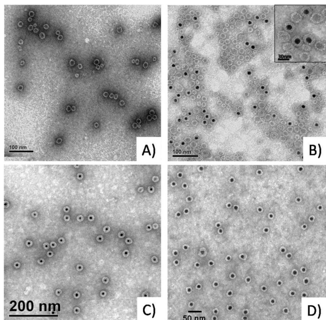
Figure 2. TEM pictures of assembly products: (A) Empty N \Delta 34 capsids showing significant size variability. (B) N \Delta 34 VLPs from an unpurified assembly reaction showing incorporation of gold cores although at a lower efficiency. Inset: higher magnification micrograph for a more detailed view of the complexes. (C) VLPs from an unpurified assembly reaction with wild-type CCMV capsid. (D) N \Delta 34 VLPs purified over a sucrose density gradient.
