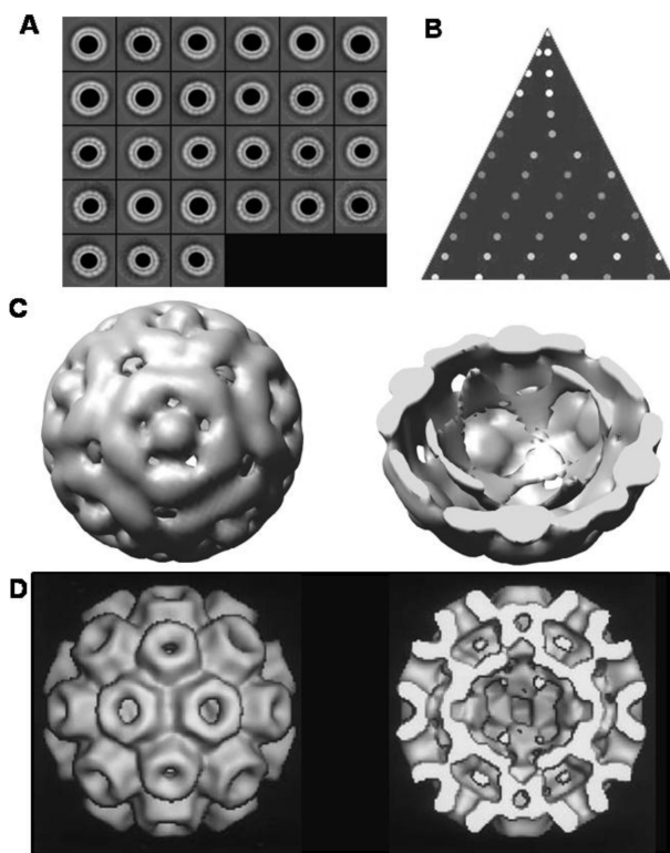
Figure 4. Negative-stain TEM reconstruction of the VLPs formed by NΔ34. (A) Class averages generated from ~3800 VLPs formed with the 11.7 nm cores. (B) An asymmetric triangle depicting anisotropy with regards to the sampling of the 3D space. (C) 3D reconstruction of the VLPs formed with 11.7 nm showing the pentamer. The surface rendering threshold was set to correspond to a molecular mass of 240 kDa. The model to the right shows a cut-away structure of the VLP. (D) The structure of the CCMV particle generated by Wikoff et al. 24
